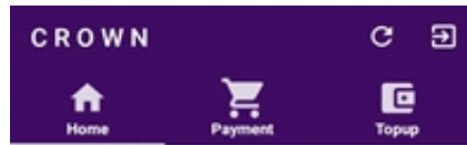
Application interface
