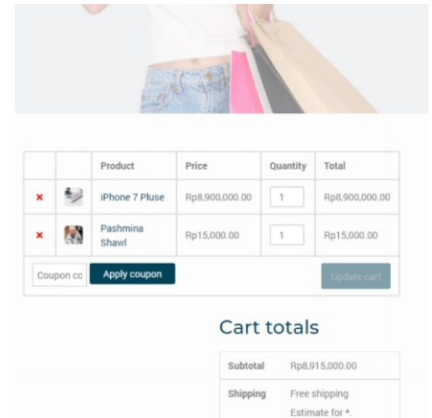
Checkout page
