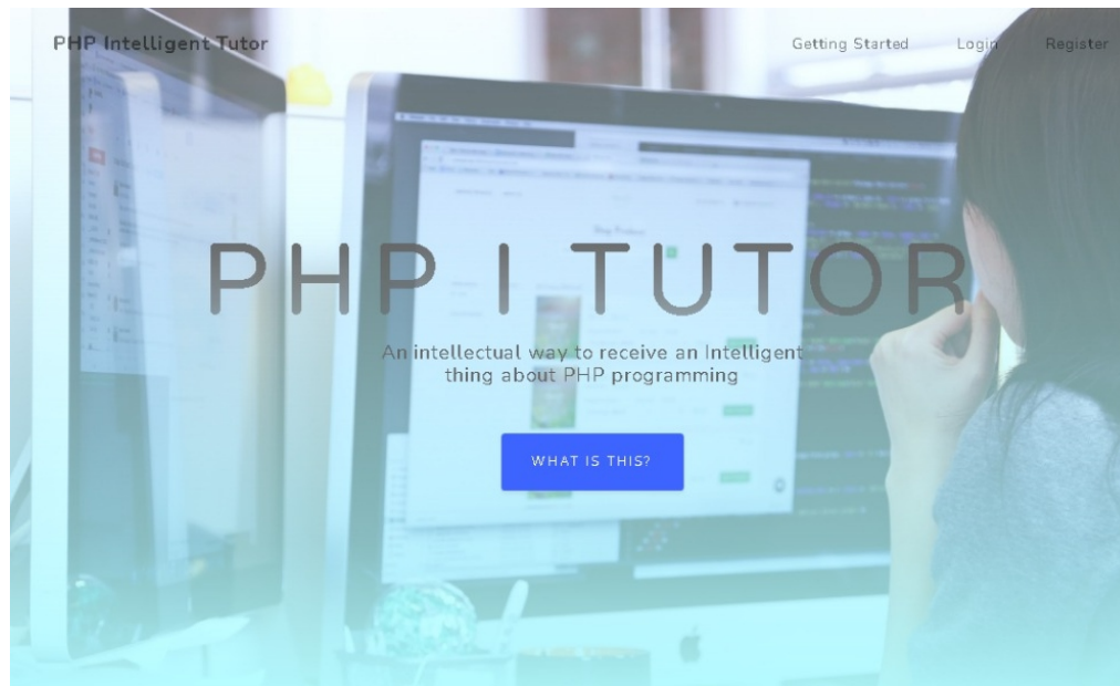
Homepage
