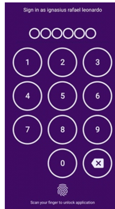
Security code
